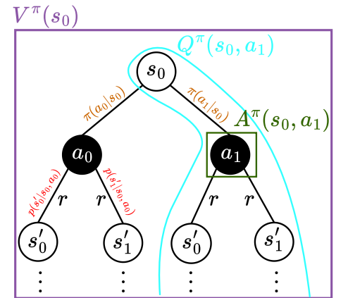
Figure 2: Backup diagram illustrating the different value functions.
